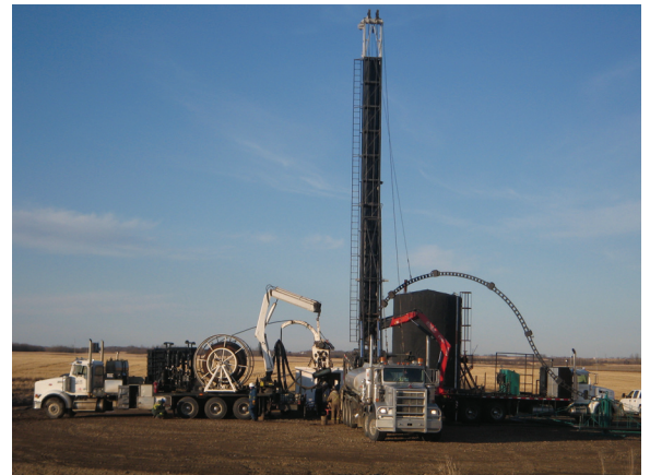
“Coil Tubing Unit, Flushby, & Truck Mounted Gripper”
